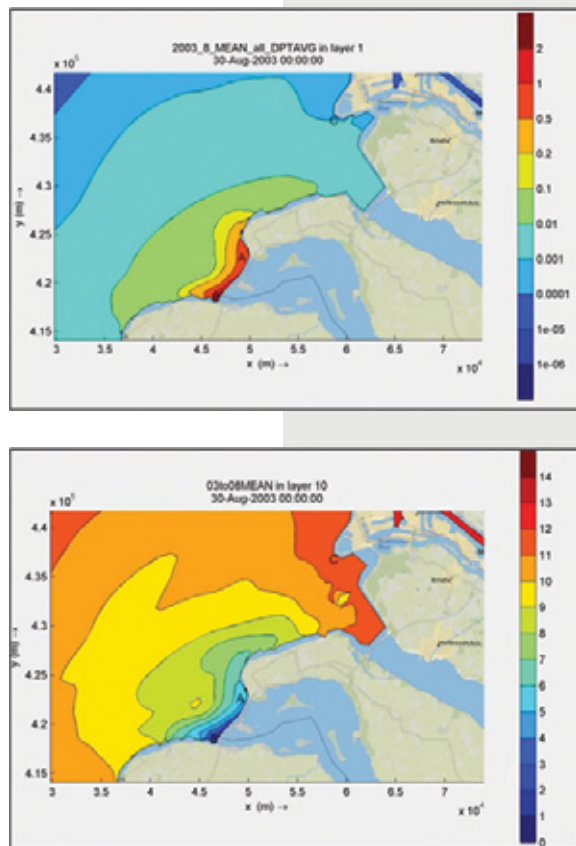
Figure 14: Model results for water dilution pattern (upper frame) and transport time (lower frame). From Kleissen 2016.
