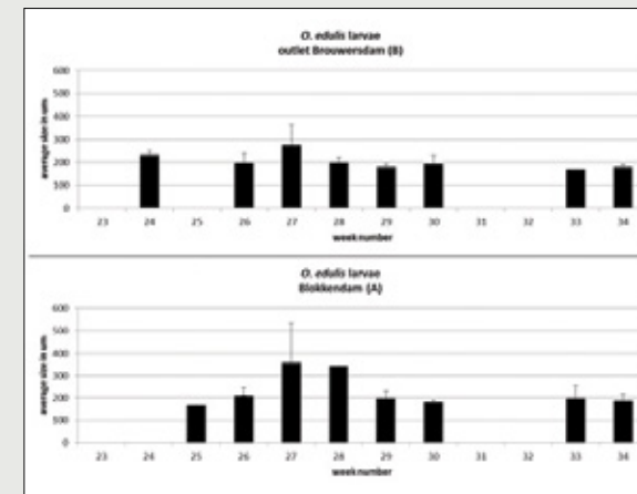
Figure 16: Average size (in µm with st. dev.) of flat oyster larvae at location B and A in 2016.
