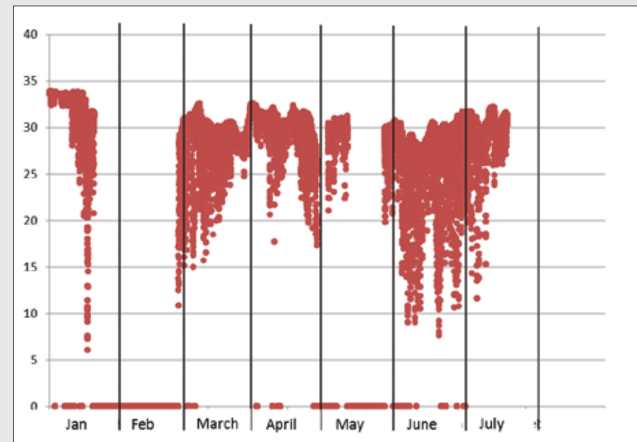
Salinity in surface water at Haringvliet mouth in 2016. Zero means no measurement. Source: Rijkswaterstaat.
